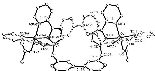
Fig. 2 Crystal structure of the complex cation of [\text{Cu}_2(\text{L}^1)_2(\text{OAc})_2][\text{BF}_4]_2 . One ligand strand is shown with hollow bonds for clarity.
