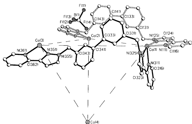
Fig. 3 Crystal structure of part of the complex cation of [\text{Co}_4(\text{L}^1)_6][\text{BF}_4]_8 \cdot 6\text{MeCN} , showing (i) the tetrahedral arrangement of metal ions, (ii) two of the six ligands which bridge the edges of the tetrahedron, and (iii) one of the [\text{BF}_4]^- anions which is involved in weak \text{CH} \cdots \text{F} hydrogen bonding interactions with the periphery of the complex cation.
